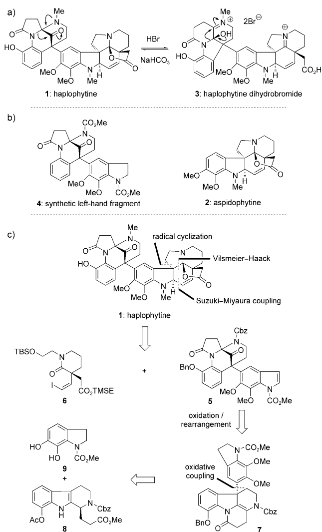
Scheme 1. Structures of haplophytine ( 1 , a), haplophytine dihydrobromide ( 3 , a), aspidophytine ( 2 , b), synthetic left-hand fragment 4 (b) and our retrosynthetic analysis of haplophytine ( 1 , c). Ac = acetyl, Bn = benzyl, Cbz = benzyloxycarbonyl, TBS = tert -butyldimethylsilyl, TMSE = trimethylsilylethyl.
